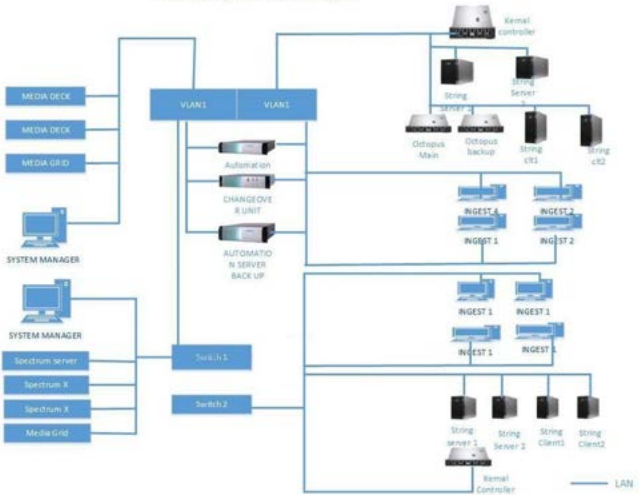
Automation general Network Diagram
